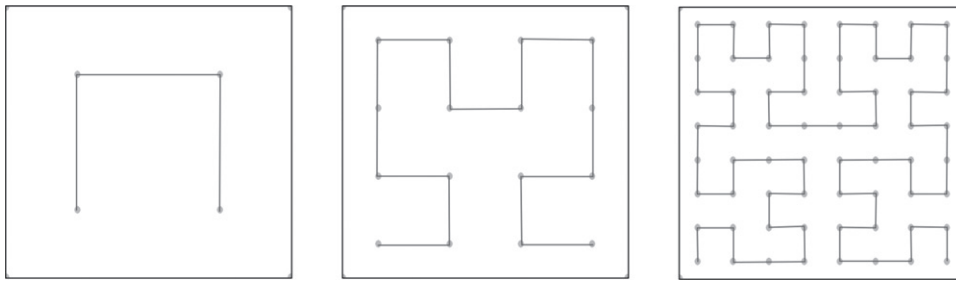
Figure 2. Illustration for the first three stages of the Hilbert's space filling curves when d = 2 . From left to right, each panel shows H_1, H_2 , and H_3 , respectively.
